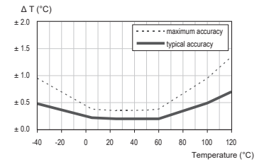
Figure 2. Maximal tolerance for temperature sensor in °C.
